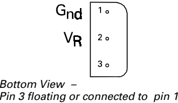
E-Line, 3 pin, Rev Package Suffix – R
