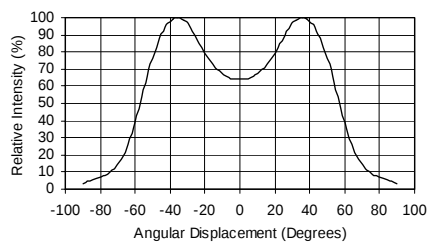
Figure 7a. Representative Spatial Radiation Pattern per Luxeon emitter White.
