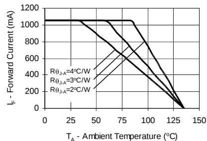
Figure 6a. Maximum Forward Current vs. Ambient Temperature. Derating based on T_{JMAX} = 135^\circ\text{C} for White, Green, Cyan and Blue18-Up.
