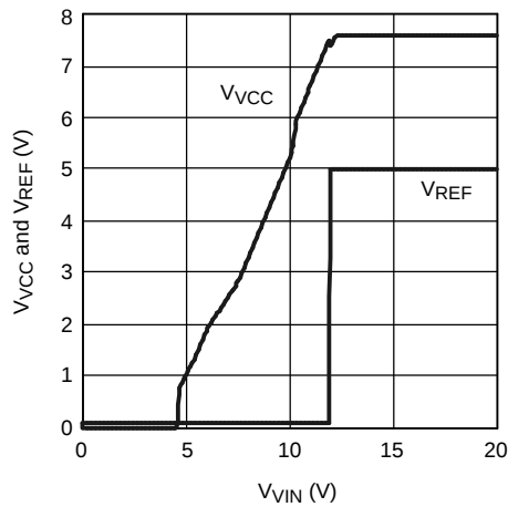
Figure 1. V_{VCC} and V_{REF} vs V_{VIN}
