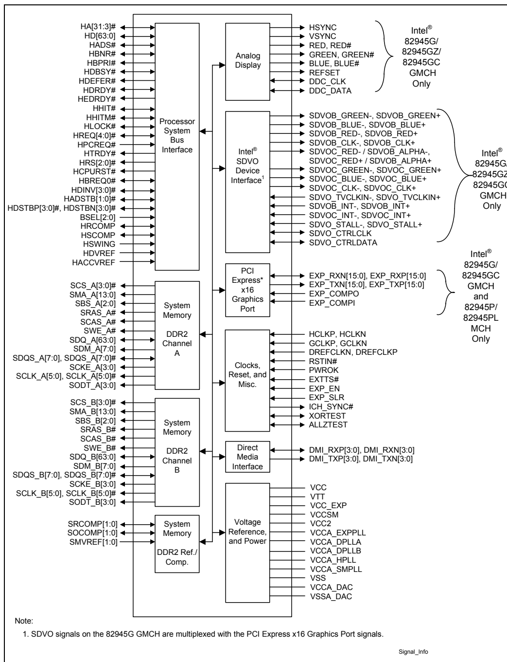
Figure 2-1. Signal Information Diagram
