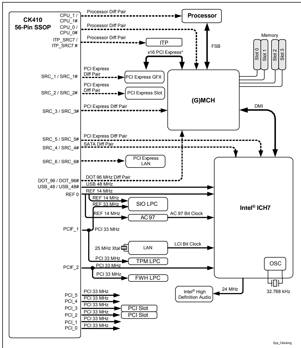
Figure 10-7. System Clocking Example
