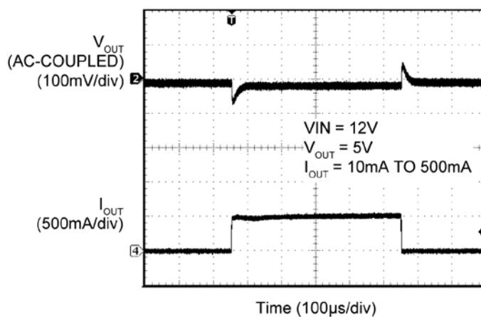
MIC28304-2 Transient Response
