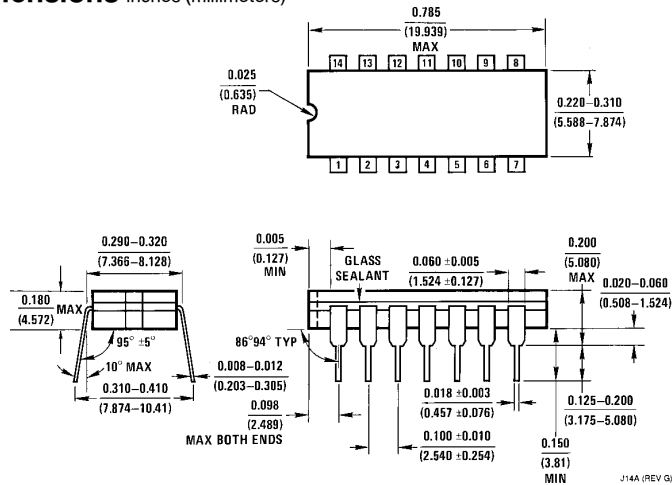
Order Number MM54HC74J or MM74HC74J NS Package J14A
