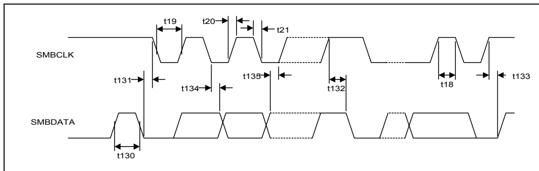
Figure 18. SMBus Transaction
