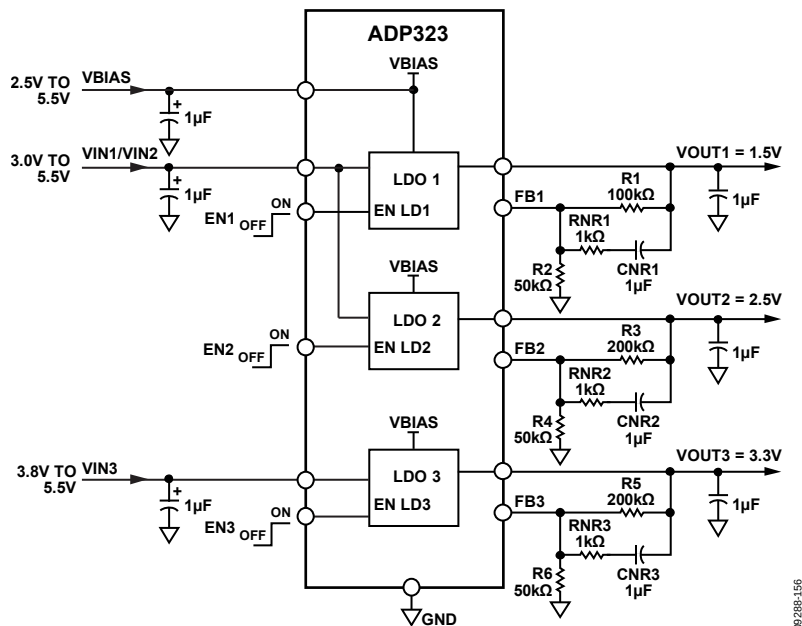
Figure 56. Noise Reduction Modification
