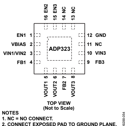
Figure 4. ADP323 Pin Configuration
