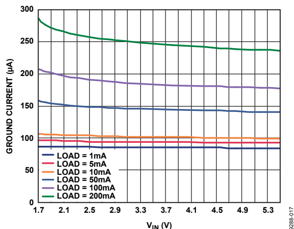
Figure 19. Ground Current vs. Input Voltage, All Outputs Loaded Equally, V_{\text{RIPPLE}} = 50 \text{ mV} , C_{\text{OUT}} = 1 \mu\text{F}
