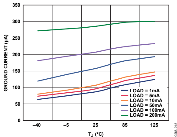
Figure 17. Ground Current vs. Junction Temperature, All Outputs Loaded Equally, V_{\text{RIPPLE}} = 50 \text{ mV} , C_{\text{OUT}} = 1 \mu\text{F}
