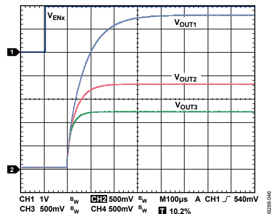
Figure 55. Typical Start-Up Time, I_{LOAD1} = I_{LOAD2} = I_{LOAD3} = 100\ \text{mA} , \text{CH1} = V_{\text{ENx}} (the Enable Voltage), \text{CH2} = V_{\text{OUT1}} , \text{CH3} = V_{\text{OUT2}} , \text{CH4} = V_{\text{OUT3}}
