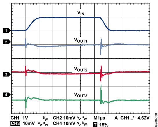
Figure 45. Line Transient Response, V_{IN} = 4\text{ V to } 5\text{ V} , I_{LOAD1} = I_{LOAD2} = I_{LOAD3} = 100\text{ mA} , CH1 = V_{IN} , CH2 = V_{OUT1} , CH3 = V_{OUT2} , CH4 = V_{OUT3} , V_{RIPPLE} = 50\text{ mV} , C_{OUT} = 1\text{ }\mu\text{F}
