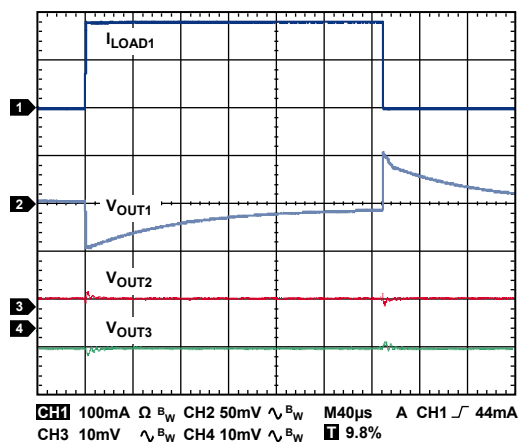
Figure 41. Load Transient Response, I_{\text{LOAD1}} = 1 \text{ mA to } 200 \text{ mA} , I_{\text{LOAD2}} = I_{\text{LOAD3}} = 1 \text{ mA} , \text{CH1} = I_{\text{LOAD1}} , \text{CH2} = V_{\text{OUT1}} , \text{CH3} = V_{\text{OUT2}} , \text{CH4} = V_{\text{OUT3}} , V_{\text{RIPPLE}} = 50 \text{ mV} , C_{\text{OUT}} = 1 \mu\text{F}
