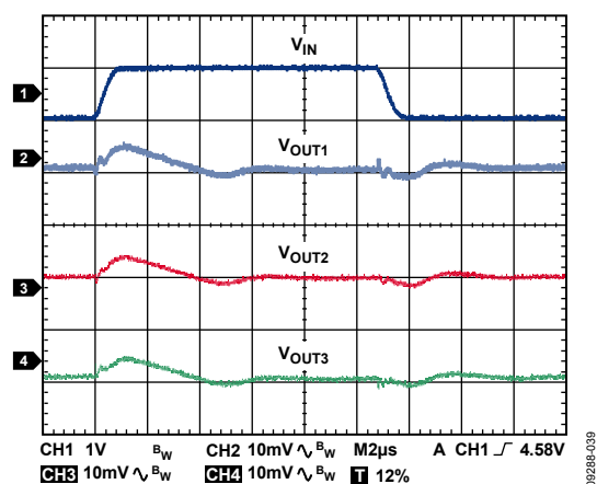
Figure 46. Line Transient Response, V_{IN} = 4\text{ V to } 5\text{ V} , I_{LOAD1} = I_{LOAD2} = I_{LOAD3} = 1\text{ mA} , CH1 = V_{IN} , CH2 = V_{OUT1} , CH3 = V_{OUT2} , CH4 = V_{OUT3} , V_{RIPPLE} = 50\text{ mV} , C_{OUT} = 1\text{ }\mu\text{F}
