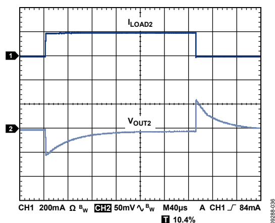
Figure 43. Load Transient Response, I_{\text{LOAD2}} = 1 \text{ mA to } 200 \text{ mA} , C_{\text{OUT2}} = 1 \mu\text{F} , \text{CH1} = I_{\text{LOAD2}} , \text{CH2} = V_{\text{OUT2}} , V_{\text{RIPPLE}} = 50 \text{ mV} , C_{\text{OUT}} = 1 \mu\text{F}
