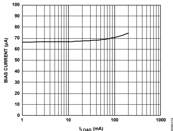
Figure 21. Bias Current vs. Load Current, Single Output Loaded, V_{\text{RIPPLE}} = 50 \text{ mV} , C_{\text{OUT}} = 1 \mu\text{F}
