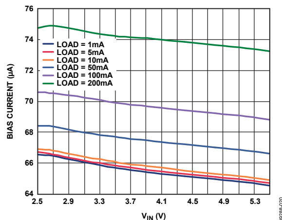
Figure 22. Bias Current vs. Input Voltage, Single Output Loaded, V_{\text{RIPPLE}} = 50 \text{ mV} , C_{\text{OUT}} = 1 \mu\text{F}
