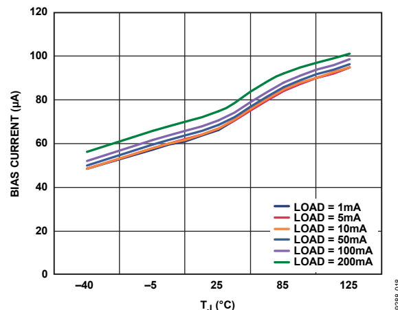
Figure 20. Bias Current vs. Junction Temperature, Single Output Loaded, V_{\text{RIPPLE}} = 50 \text{ mV} , C_{\text{OUT}} = 1 \mu\text{F}
