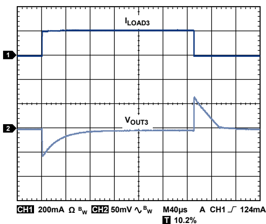
Figure 44. Load Transient Response, I_{\text{LOAD3}} = 1 \text{ mA to } 200 \text{ mA} , C_{\text{OUT3}} = 1 \mu\text{F} , \text{CH1} = I_{\text{LOAD3}} , \text{CH2} = V_{\text{OUT3}} , V_{\text{RIPPLE}} = 50 \text{ mV} , C_{\text{OUT}} = 1 \mu\text{F}
