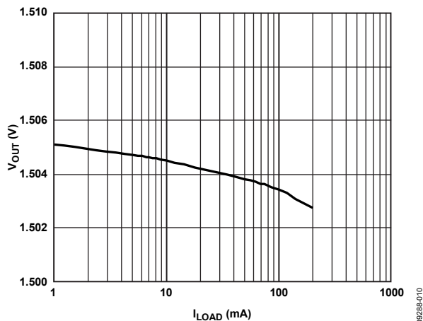
Figure 12. Output Voltage vs. Load Current, V_{\text{RIPPLE}} = 50 \text{ mV} , C_{\text{OUT}} = 1 \mu\text{F}
