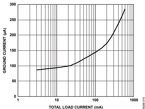
Figure 18. Ground Current vs. Load Current, All Outputs Loaded Equally, V_{\text{RIPPLE}} = 50 \text{ mV} , C_{\text{OUT}} = 1 \mu\text{F}
