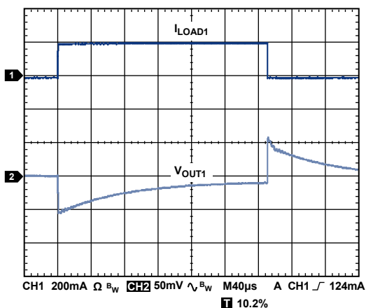
Figure 42. Load Transient Response, I_{\text{LOAD1}} = 1 \text{ mA to } 200 \text{ mA} , C_{\text{OUT1}} = 1 \mu\text{F} , \text{CH1} = I_{\text{LOAD1}} , \text{CH2} = V_{\text{OUT1}} , V_{\text{RIPPLE}} = 50 \text{ mV} , C_{\text{OUT}} = 1 \mu\text{F}
