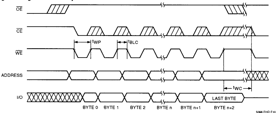
Figure 6. Page Mode Write Cycle
