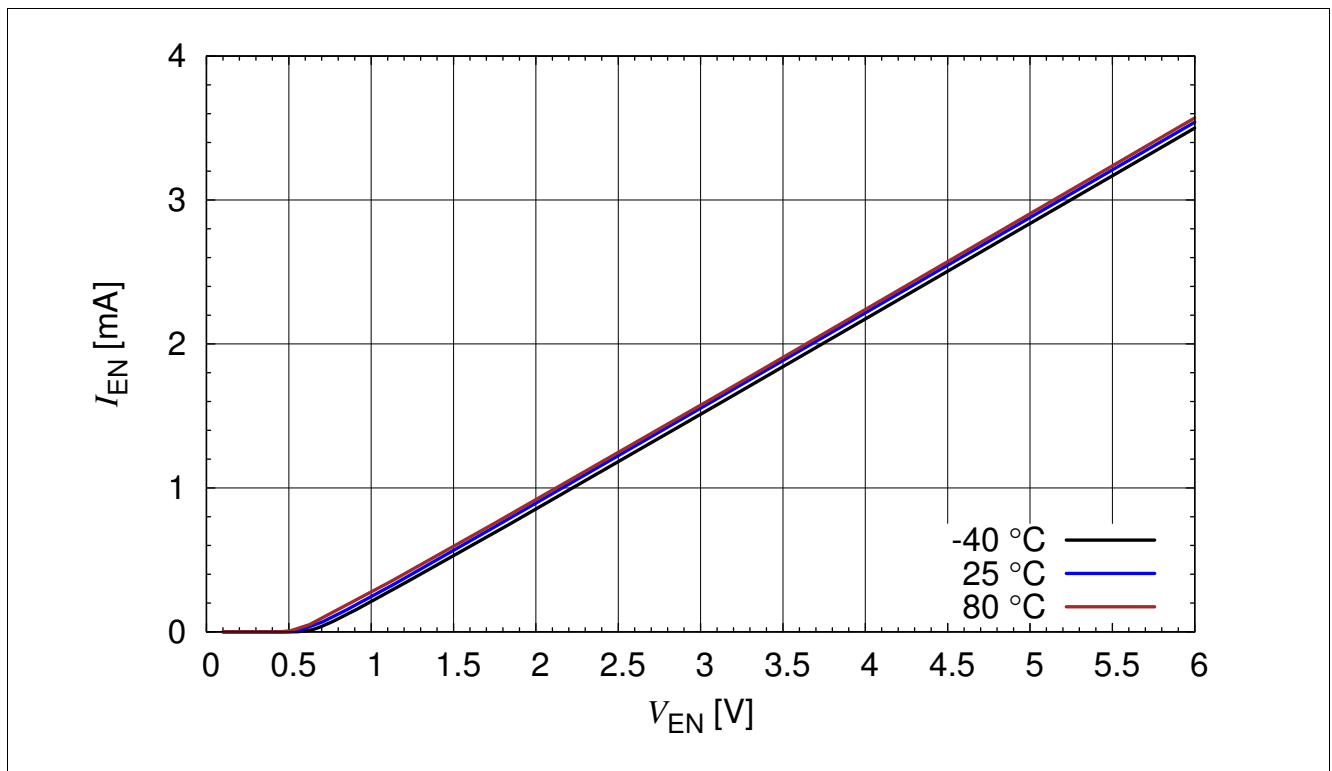
Figure 3-23 BCR321U: Enable Current versus V_{EN} I_{EN} = f(V_{EN}) , R_{ext} = \text{open} , I_{out} = 0 A, T_A = Parameter
