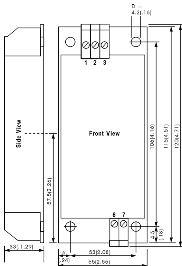
Pin-Out
