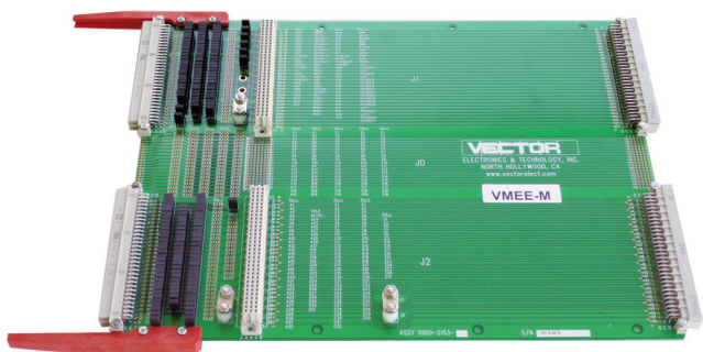
VMEE-M (6U, VME J1/J2 w/3-row, 96-pin connectors)
