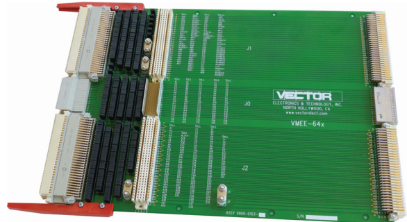
VME64-M (6U, VME64x J1/J2/J0)
