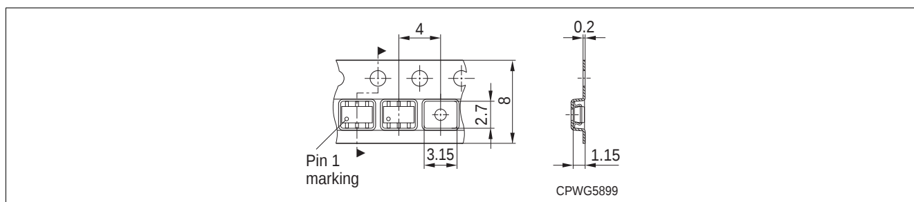
Figure 6 Tape loading
