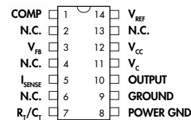
J & N PACKAGE (Top View)
