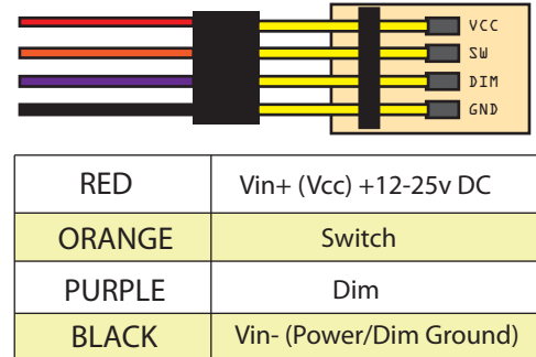
Fig. 1 - Electrical Connections
