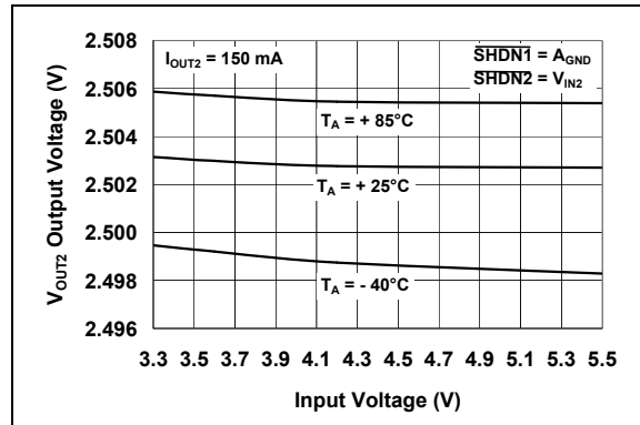
FIGURE 2-24: V_{OUT2} Output Voltage vs. Input Voltage ( V_{OUT2} = 2.5V ).
