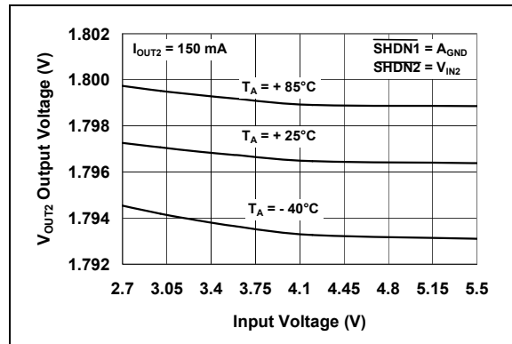
FIGURE 2-23: V_{OUT2} Output Voltage vs. Input Voltage ( V_{OUT2} = 1.8V ).
