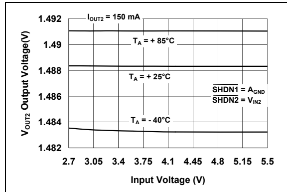
FIGURE 2-22: V_{OUT2} Output Voltage vs. Input Voltage ( V_{OUT2} = 1.5V ).
