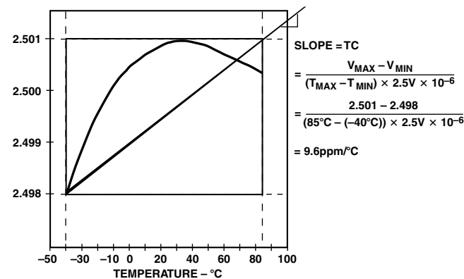
Figure 9. Typical AD680AN/AP Temperature Drift
