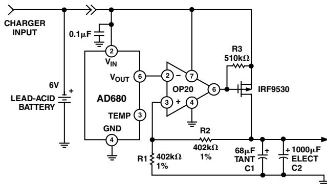
The AD680 is ideal for providing a stable, low cost and low power reference voltage in portable equipment power supplies. Figure 14 shows how the AD680 can be used in a voltage regulator that not only has low output noise (as compared to a switch mode design) and low power, but also a very fast recovery after current surges. Some precaution should be taken in the selection of the output capacitors. Too high an ESR (effective series resistance) could endanger the stability of the circuit. A solid tantalum capacitor, 16 V or higher, and an aluminum electrolytic capacitor, 10 V or higher, are recommended for C1 and C2, respectively. Also, the path from the ground side of C1 and C2 to the ground side of R1 should be kept as short as possible.
