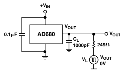
Figure 7a. Capacitive Load Transient Response Test Circuit
