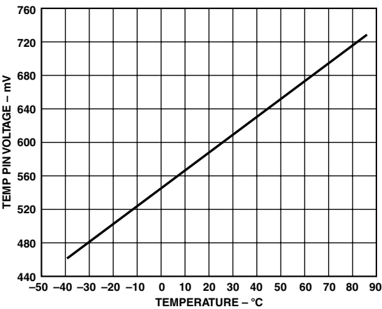
Figure 10. Temp Pin Transfer Characteristic
