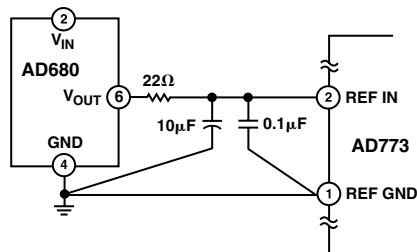
Figure 12b shows the AD680 connected to the AD773 high speed 8-bit ADC. The low-pass filter shown minimizes the AD680's wideband noise.
