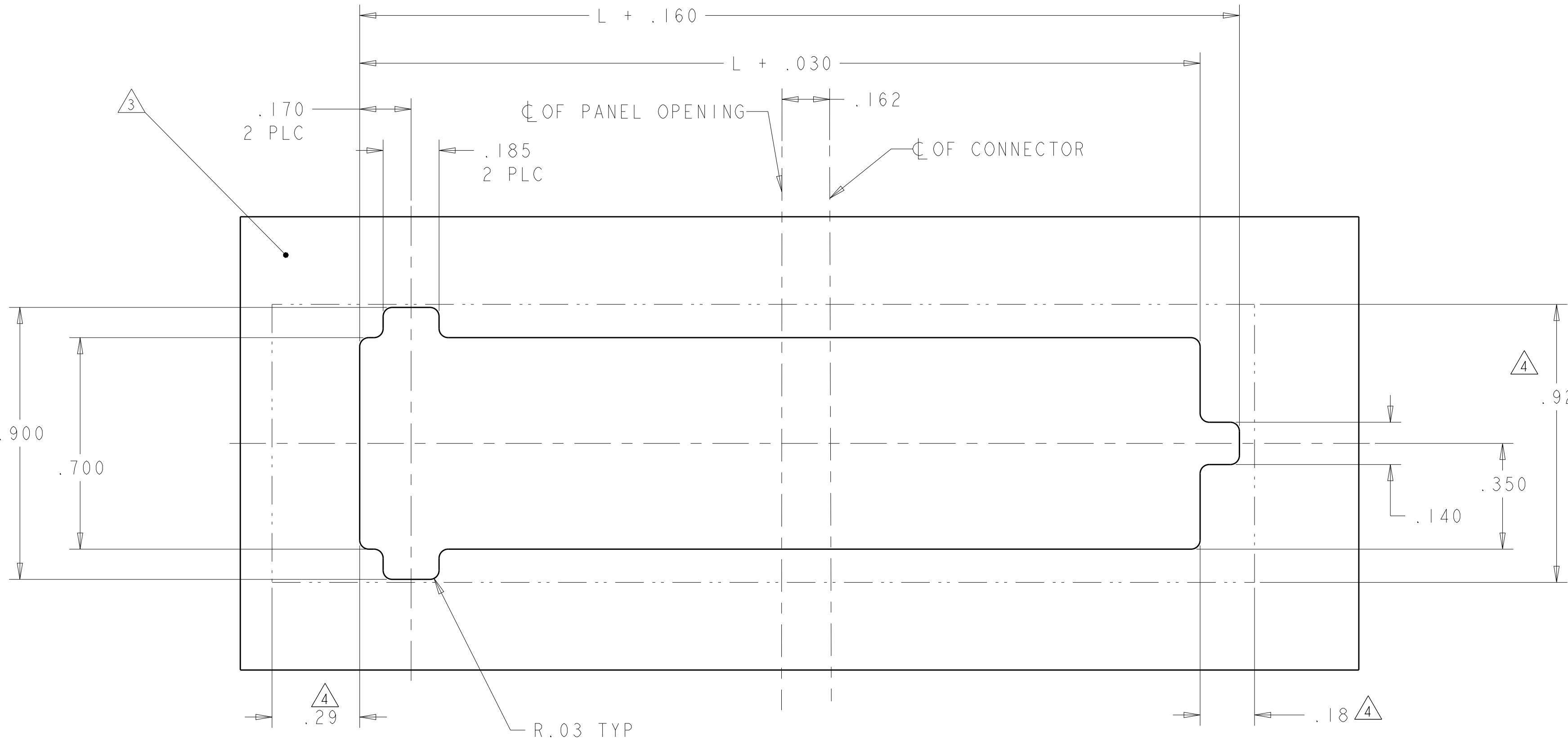
PANEL LAYOUT
