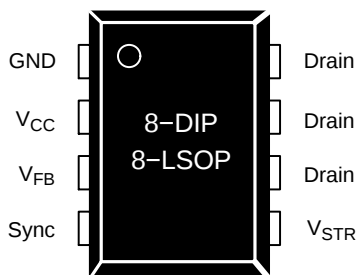
Figure 3. Pin Configuration (Top View)
