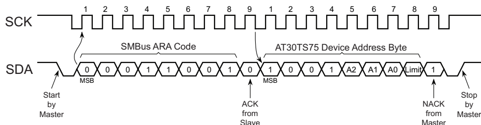
Figure 7-1. SMBus Alert
