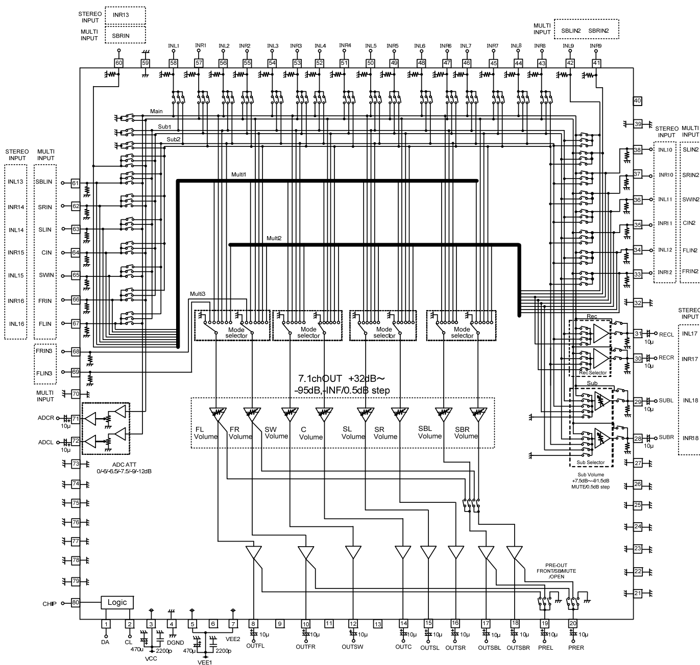
Figure 17. Application Circuit Diagram
