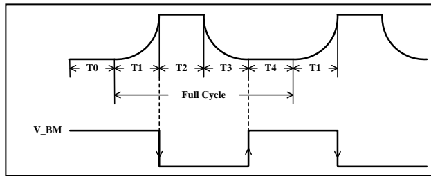
Figure 8 V_BM Signal
