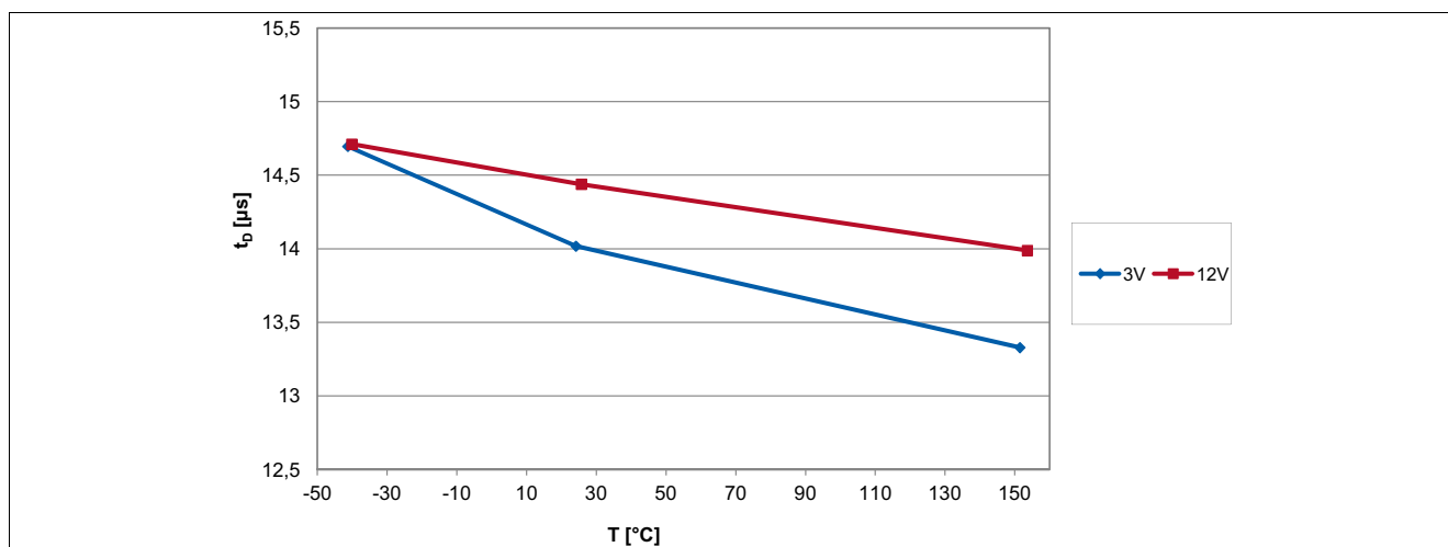
Figure 6-2 Signal Delay Time of the TLE4964-3M over Temperature
