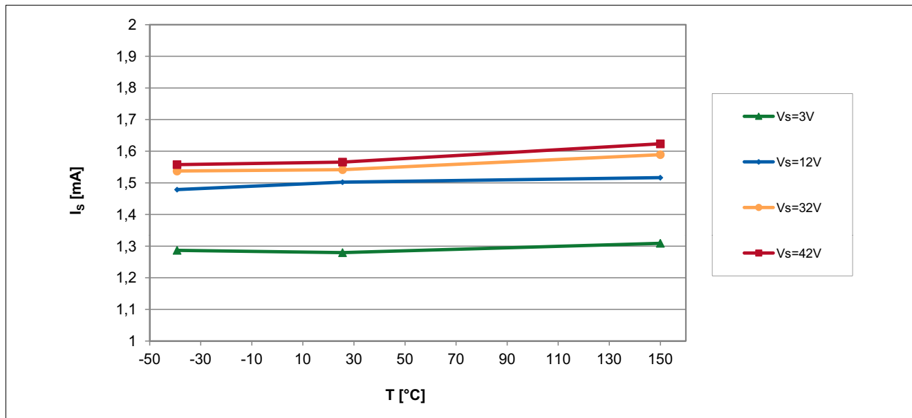
Figure 6-3 Supply Current of the TLE4964-3M over Temperature
