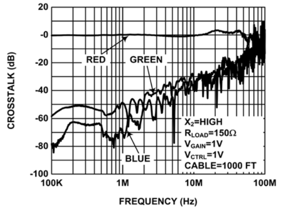
FIGURE 20. RED CROSSTALK
