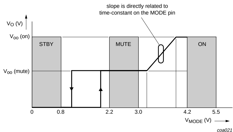
Fig 7. Behavior of mode selection pin MODE.
