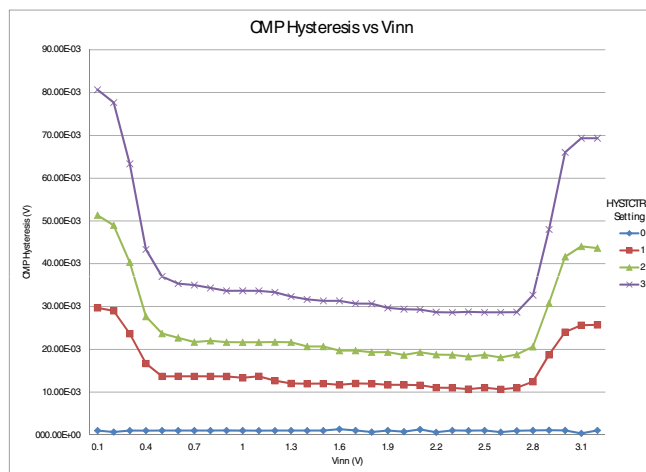
Figure 9. Typical hysteresis vs. Vin level ( V_{DD} = 3.3\text{ V} , PMODE = 0 )
