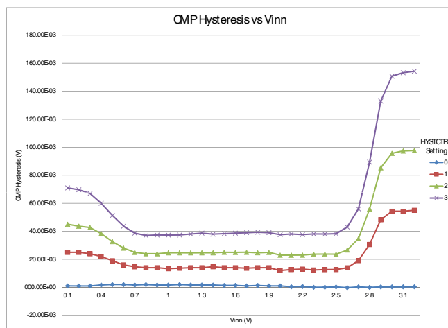
Figure 10. Typical hysteresis vs. Vin level ( V_{DD} = 3.3\text{ V} , PMODE = 1 )
