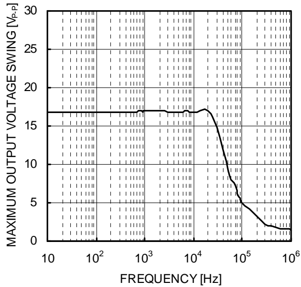
Figure 22. Maximum Output Voltage Swing – Frequency ( V_{CC}/V_{EE}=+15V/-15V , R_L=2k\Omega , T_a=25^\circ\text{C} )
