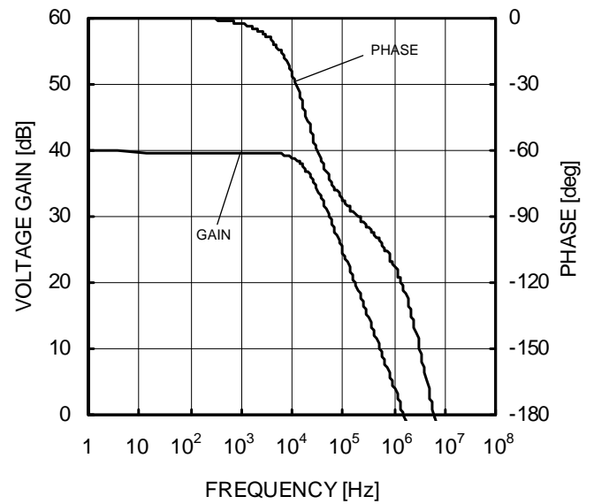
Figure 23. Voltage Gain, Phase - Frequency ( V_{CC}/V_{EE}=+15V/-15V , A_v=40\text{dB} , R_L=2k\Omega , T_a=25^\circ\text{C} )
