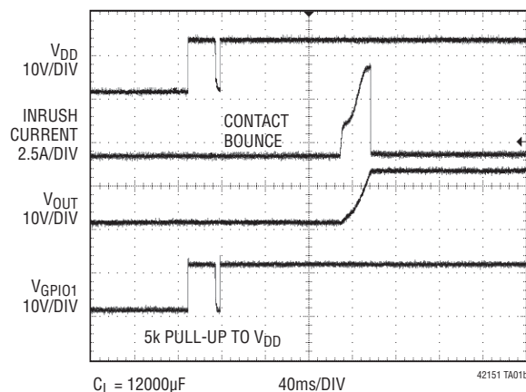
Start-Up Waveform
