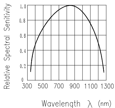
Fig.5 Spectral Sensitivity
