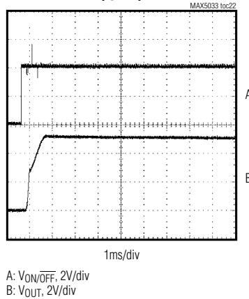
MAX5033BASA STARTUP WAVEFORM ( I_O = 0 )
