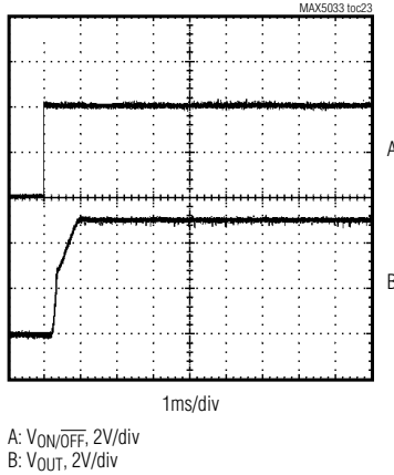
MAX5033BASA STARTUP WAVEFORM ( I_O = 0.5A )
