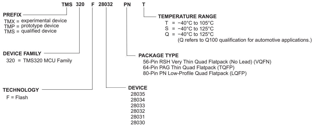
Figure 8-1. Device Nomenclature
