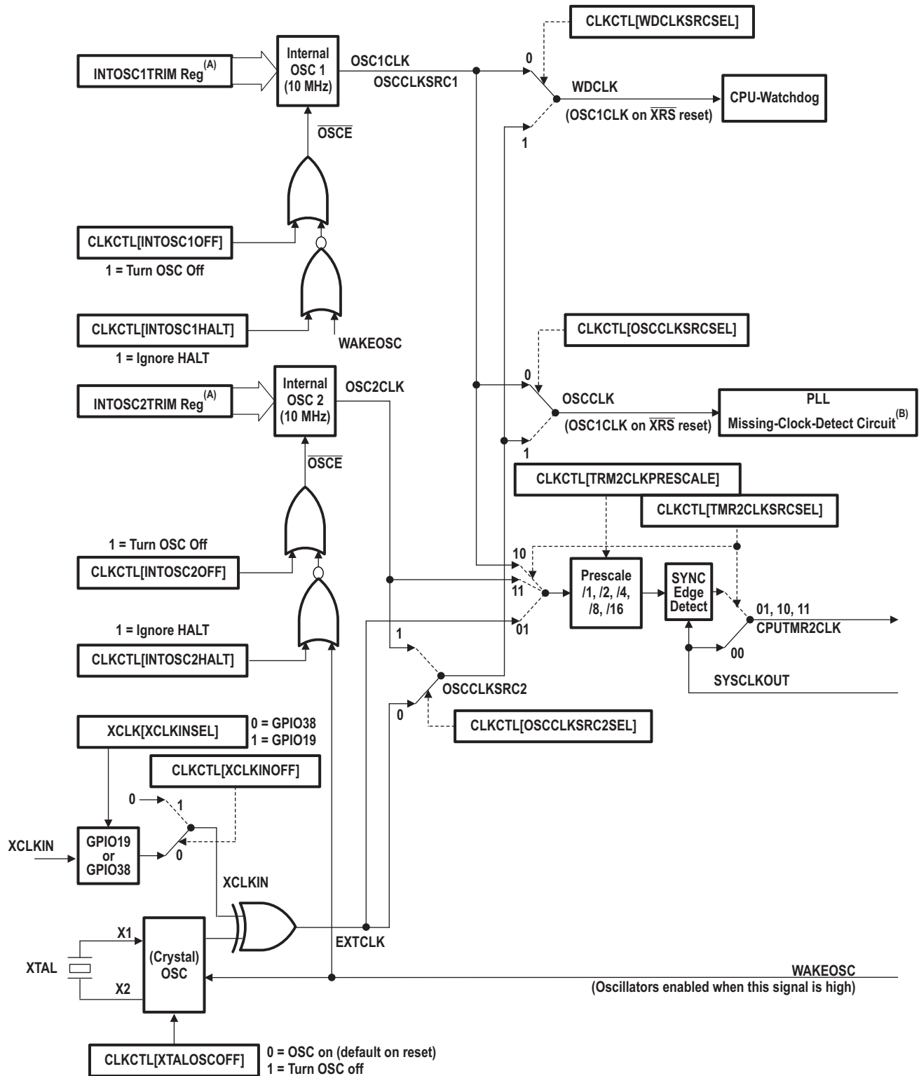
Figure 6-7. Clock Tree
