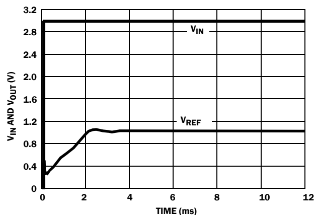
FIGURE 12. TURN-ON TIME (+25°C)
