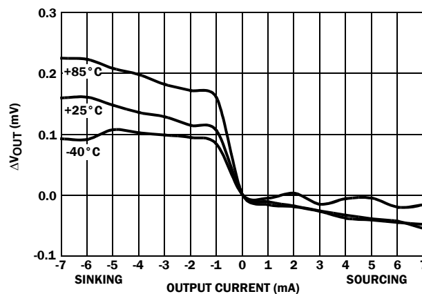
FIGURE 36. LOAD REGULATION
