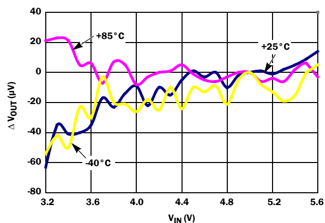
FIGURE 87. LINE REGULATION OVER-TEMPERATURE
