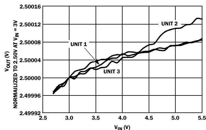
FIGURE 72. LINE REGULATION, 3 UNITS
