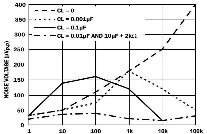
FIGURE 117. NOISE REDUCTION
