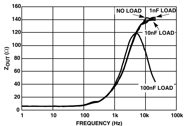
FIGURE 97. Z_{OUT} vs FREQUENCY
