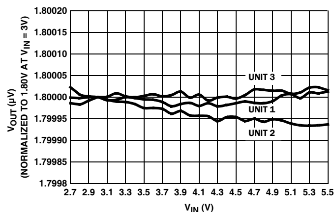
FIGURE 44. LINE REGULATION (3 REPRESENTATIVE UNITS)
