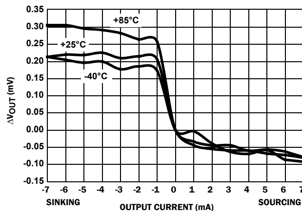
FIGURE 91. LOAD REGULATION OVER-TEMPERATURE
