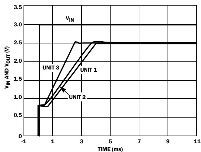
FIGURE 119. TURN-ON TIME
