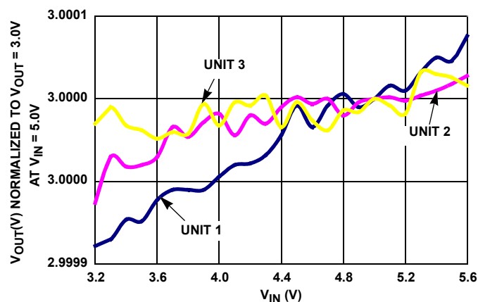
FIGURE 86. LINE REGULATION (3 REPRESENTATIVE UNITS)
