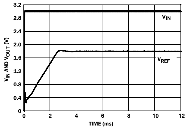
FIGURE 53. TURN-ON TIME (+25°C)
