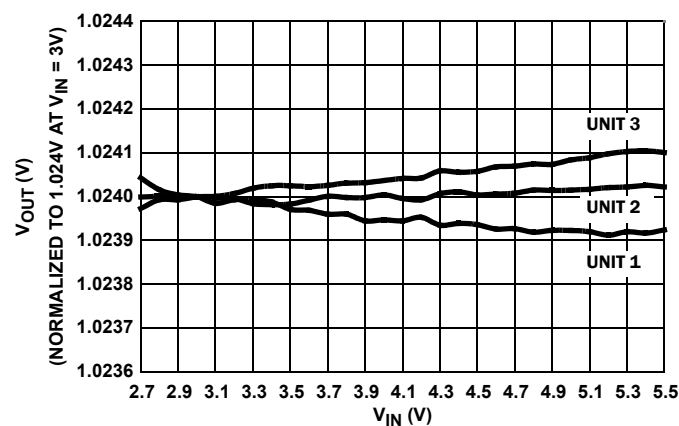
FIGURE 3. LINE REGULATION, 3 UNITS
