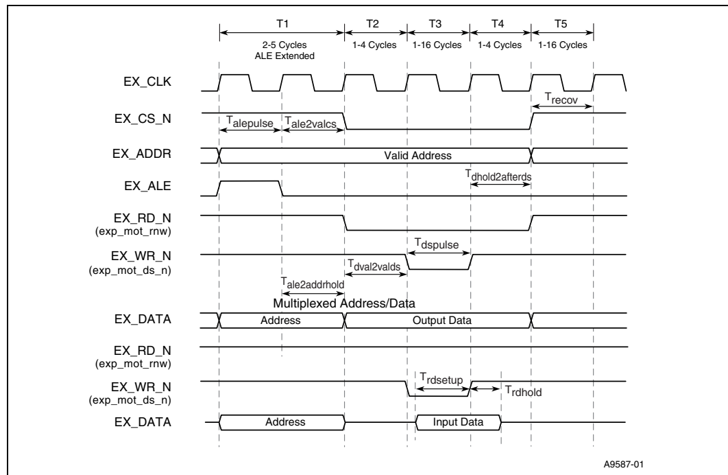
Figure 27. Motorola* Multiplexed Mode
