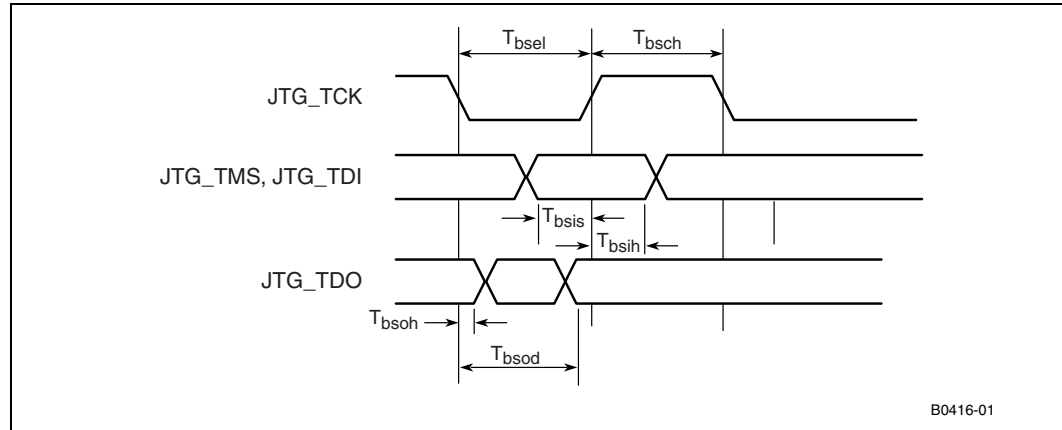
Figure 36. Boundary-Scan Reset Timings
