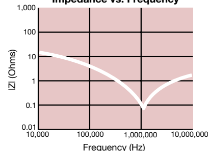
1 \mu\text{F} - 1206 Impedance vs. Frequency
