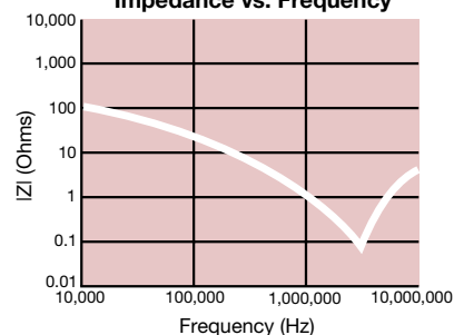
0.1 \mu\text{F} - 0603 Impedance vs. Frequency
