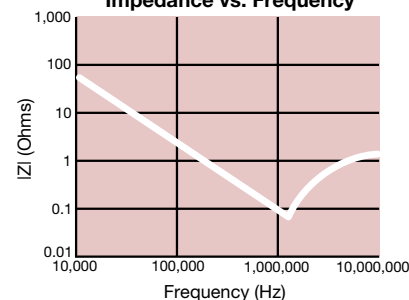
0.22 \mu\text{F} - 0805 Impedance vs. Frequency
