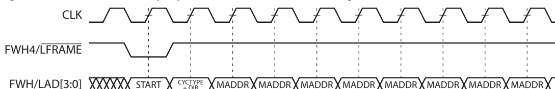
Figure 7-4. LPC Memory Cycle Initiation and Addressing
