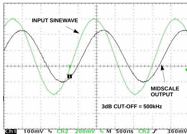
FIGURE 12. FREQUENCY RESPONSE (500kHz)
