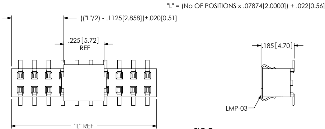
FIG 7 -M: METAL PICK & PLACE PAD ONLY AVAILABLE ON -DV (MMS-140-02-XXX-DV-M SHOWN) (DIFFERENT AS SHOWN, OTHERWISE SAME AS FIG 1)
