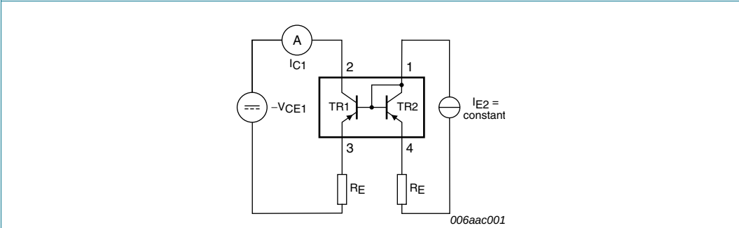
Fig 15. Current mirror with emitter resistors
