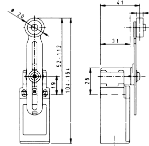
Actuator type 55 Adjustable roller-lever
