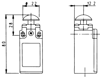
Actuator type 14 Mushroom head plunger (red plastic)
