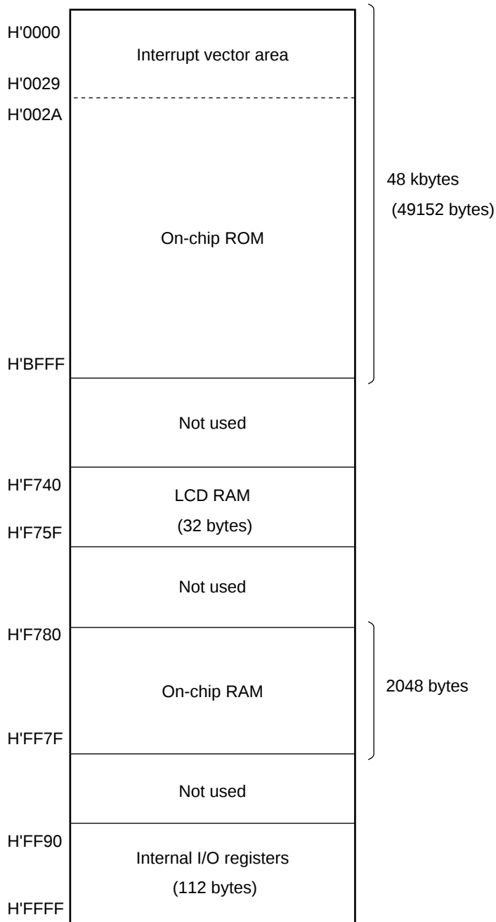
Figure 2.16 (5) H8/3846R and H8/3846S Memory Map
