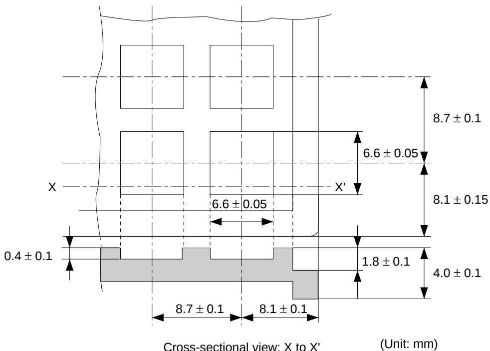
Figure I.1 Specifications of Chip Tray
