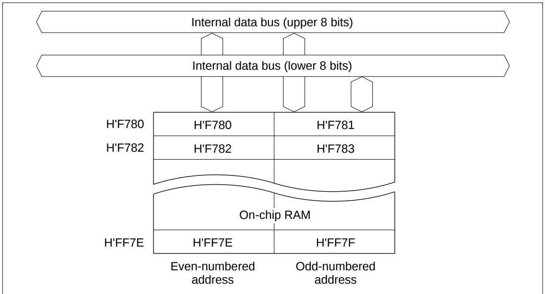
Figure 7.1 RAM Block Diagram (H8/3844R and H8/3844S)
