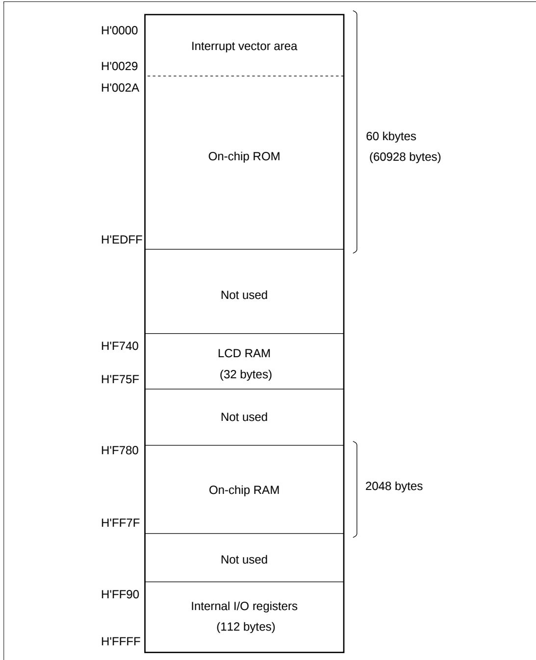
Figure 2.16 (6) H8/3847R and H8/3847S Memory Map
