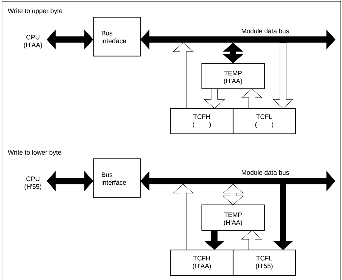
Figure 9.4 Write Access to TCR (CPU → TCF)
