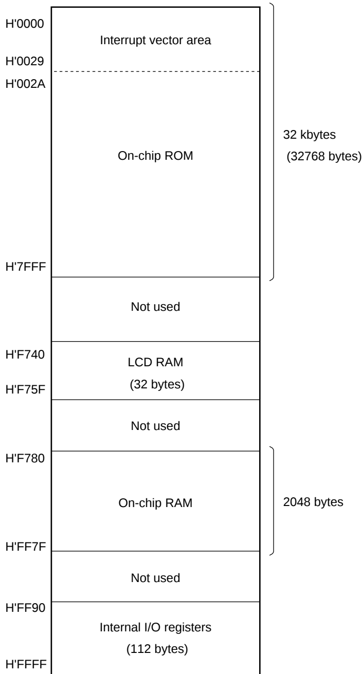
Figure 2.16 (3) H8/3844R and H8/3844S Memory Map
