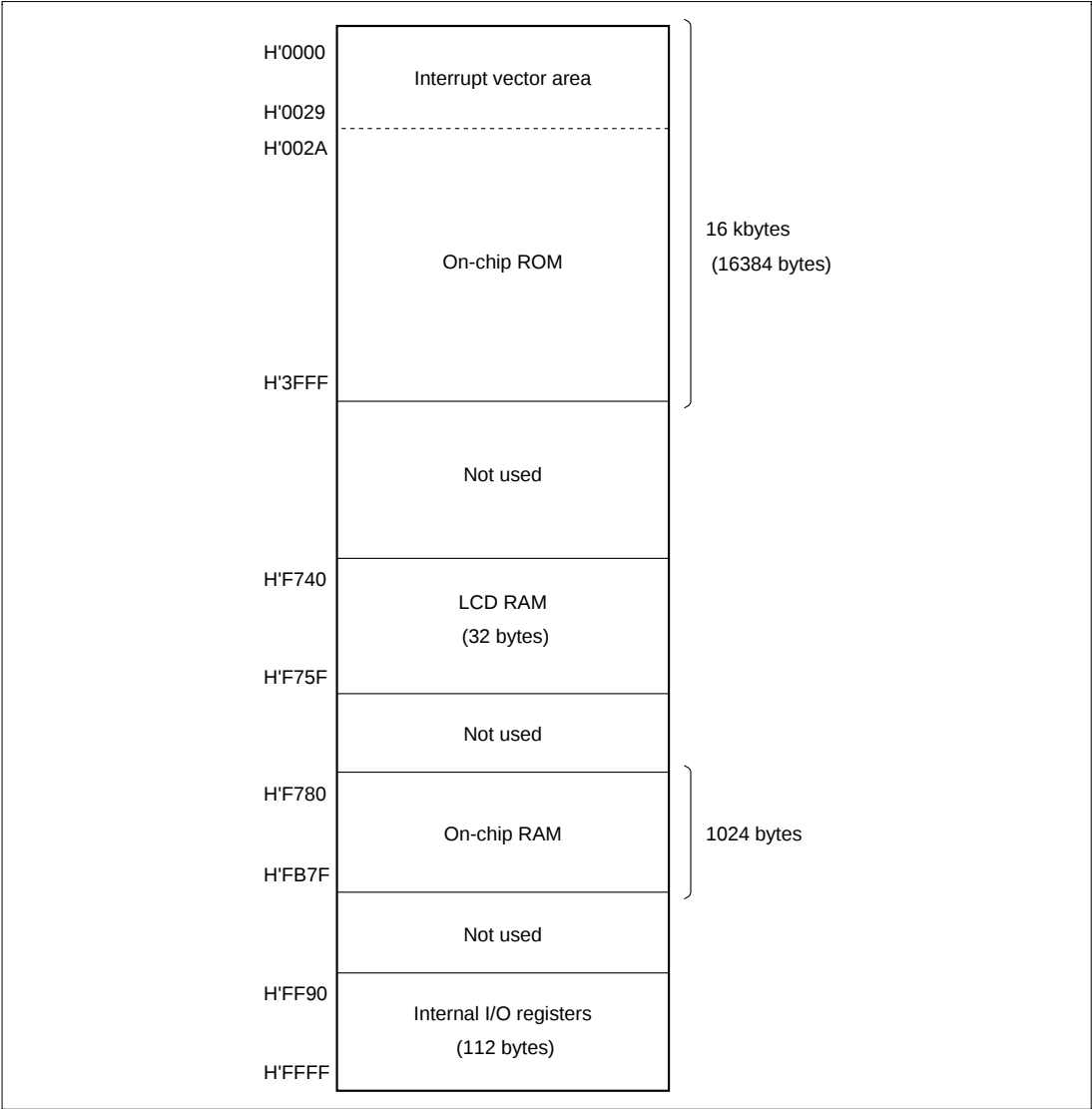
Figure 2.16 (1) H8/3842R Memory Map
