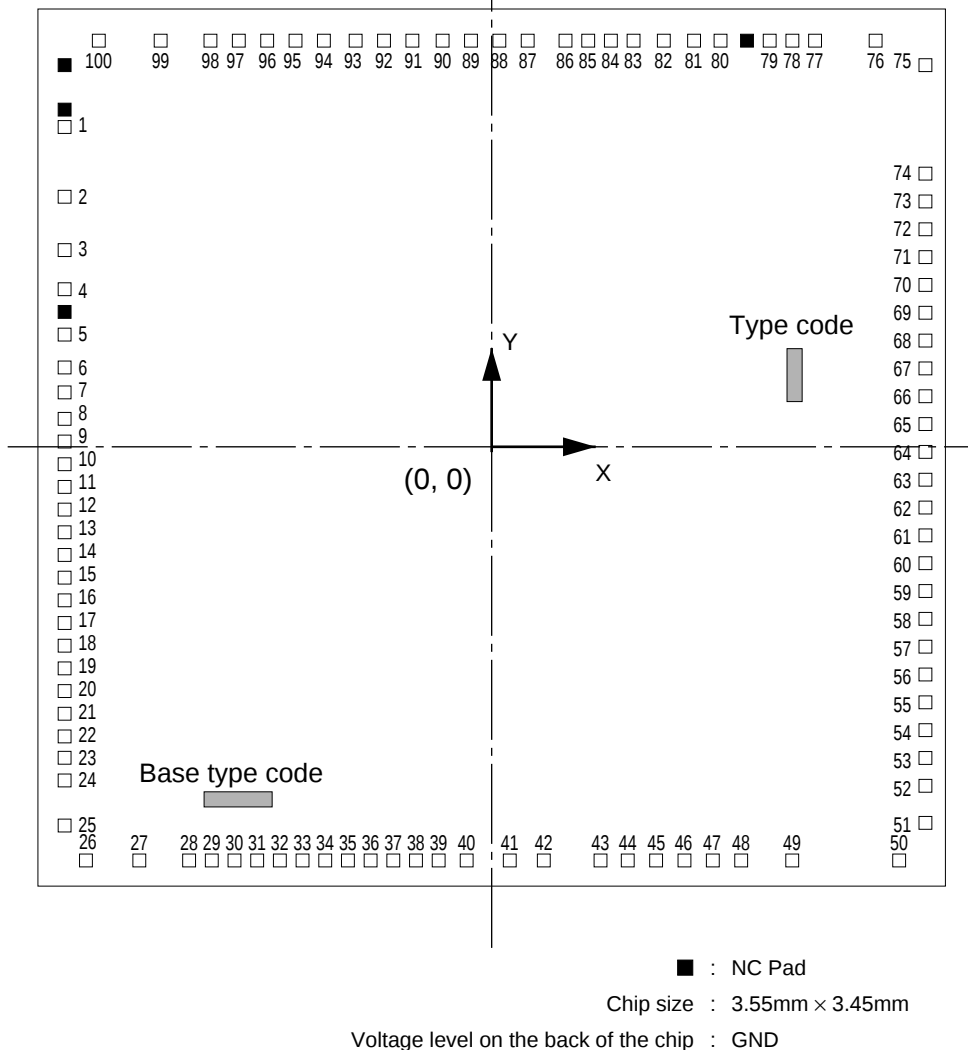
Figure 1.5 Bonding Pad Location Diagram of HCD6433847S, HCD6433846S, HCD6433845S, and HCD6433844S (Top View)
