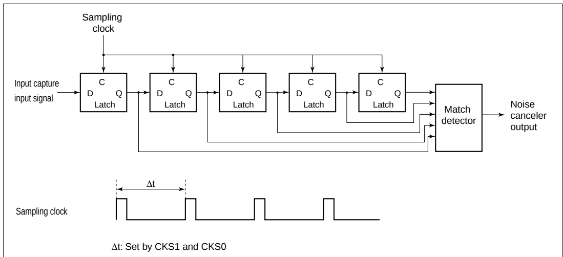
Figure 9.9 Noise Canceler Block Diagram
