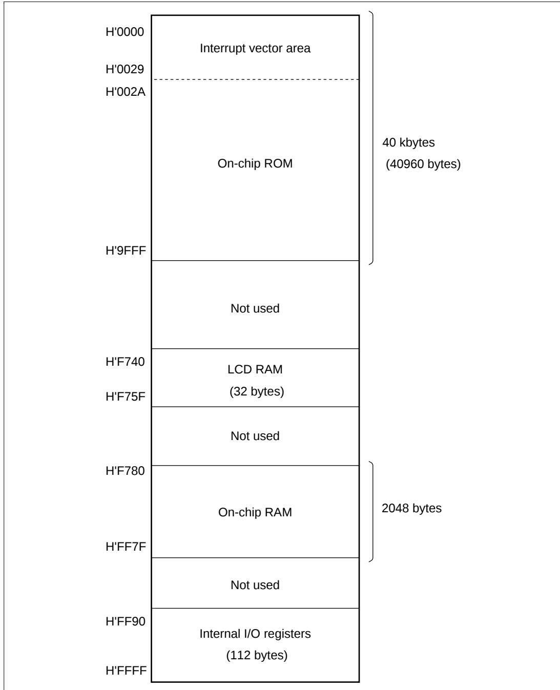
Figure 2.16 (4) H8/3845R and H8/3845S Memory Map
