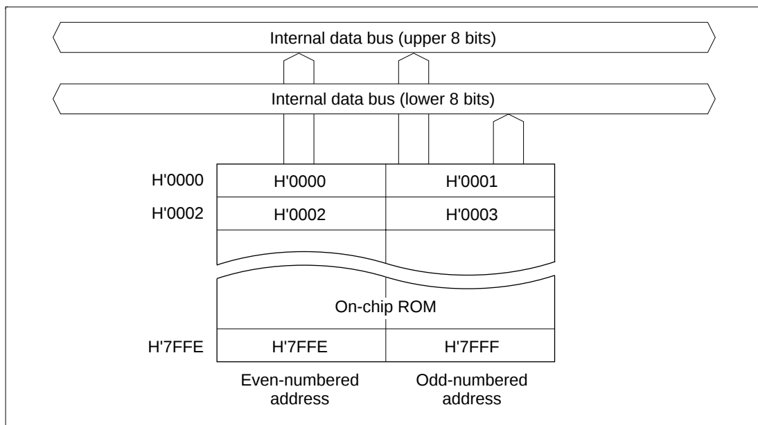
Figure 6.1 ROM Block Diagram (H8/3844R and H8/3844S)
