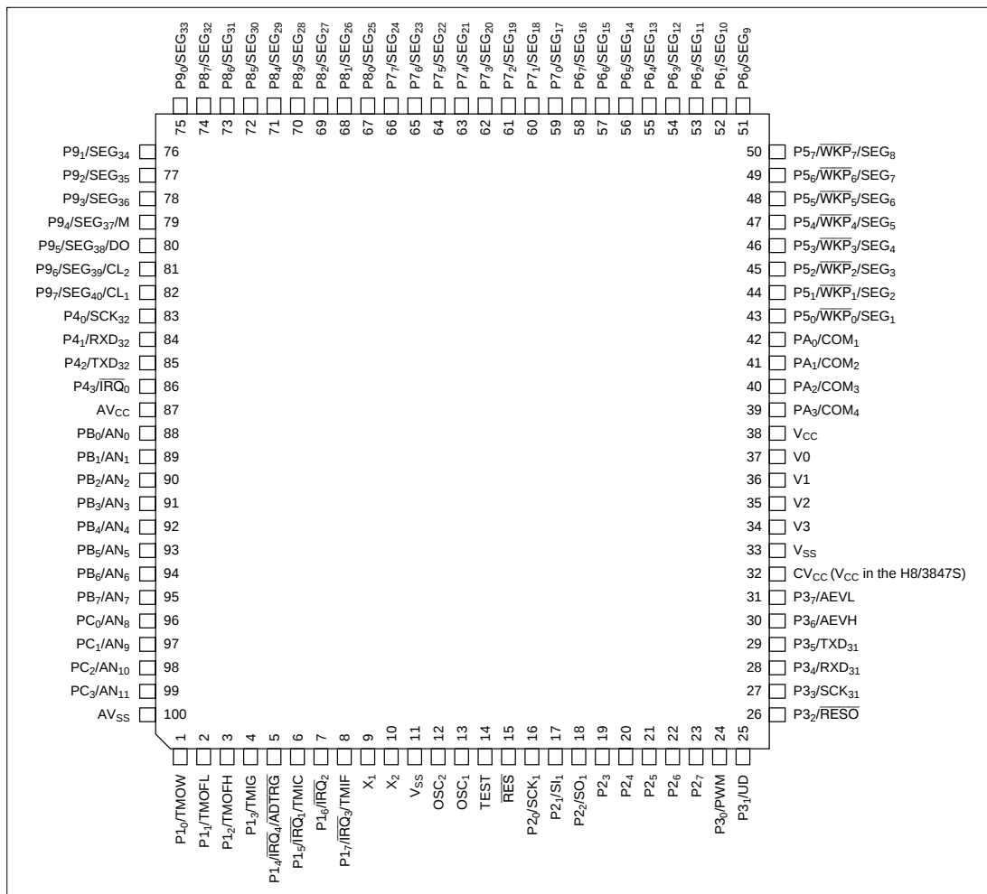
Figure 1.2 Pin Arrangement (FP-100B, TFP-100B and TFP-100G: Top View)
