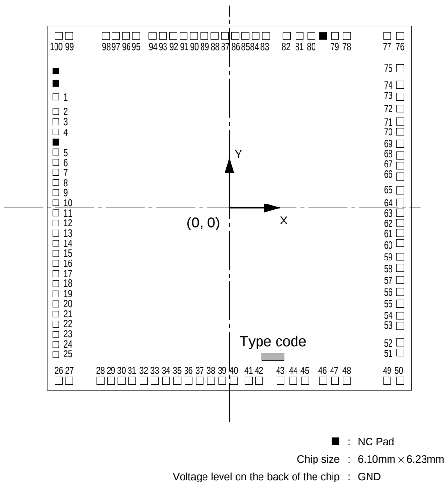
Figure 1.4 Bonding Pad Location Diagram of HCD6433847R, HCD6433846R, HCD6433845R, HCD6433844R, HCD6433843R, and HCD6433842R (Top View)
