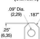
S 2 Solder Eye & Quick Connect (Standard)
