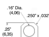
S 6 Solder Eye, extra large & quick connect
