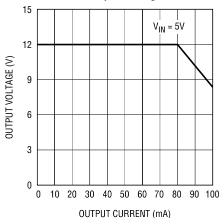
Output Voltage
