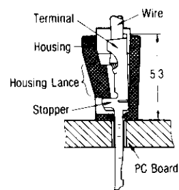
Cross View of PC Board Mount
