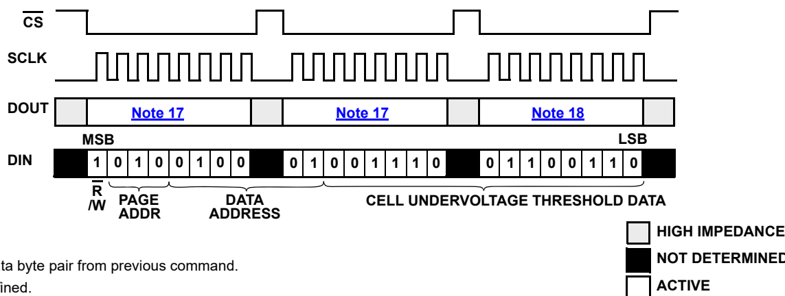
Figure 66. SPI Full Duplex (Stand-Alone) Command Example: WRITE Undervoltage Threshold Data
