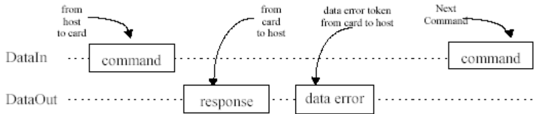
Figure 12: Read operation - data error
