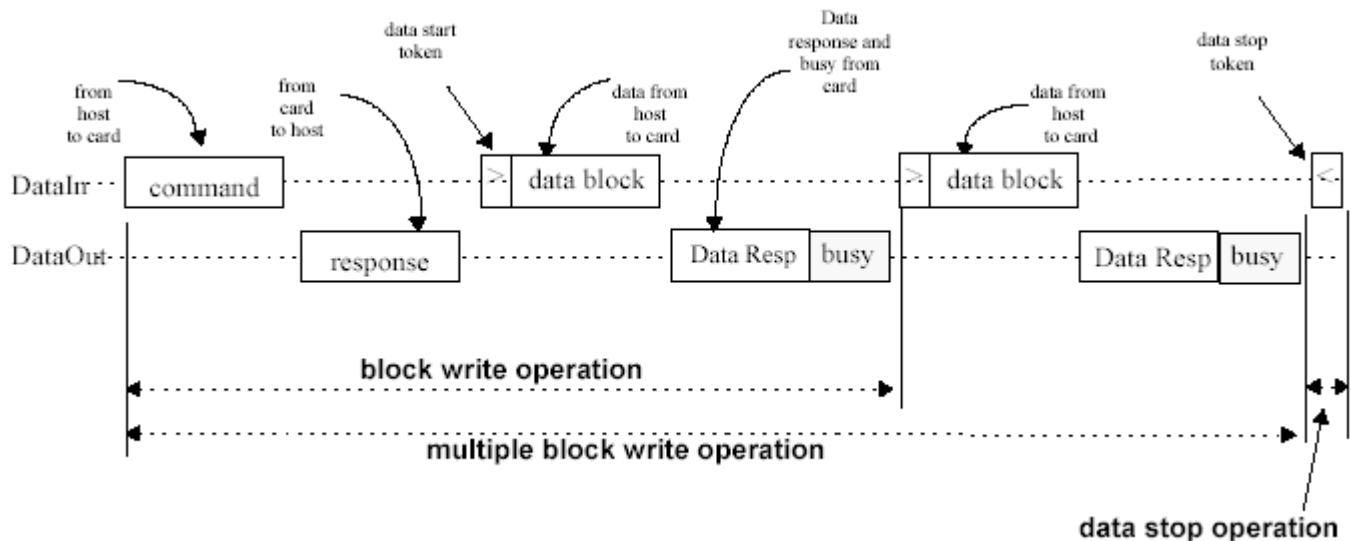
Figure 13: Write operation
