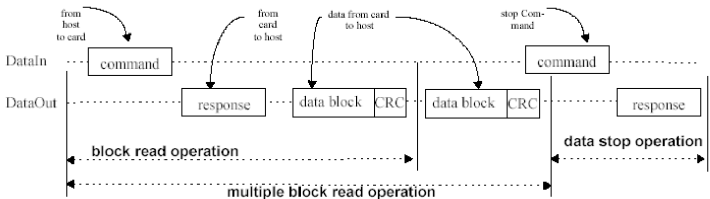
Figure 11: Read operation
