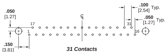
31 Contacts
