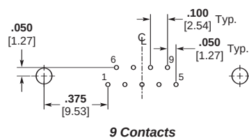
9 Contacts
