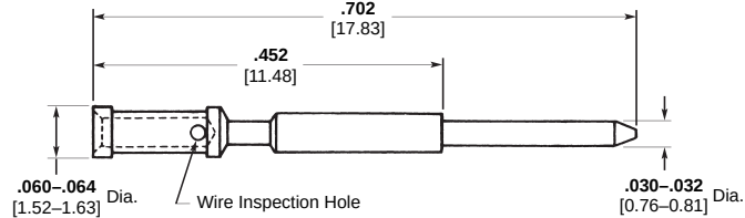
Part Number 083-0009-00R4 (6-1532030-1) 22 AWG Pin
