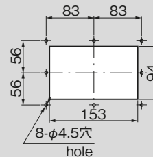
パネル穴明け寸法(1/2) Panel drilling dimension
