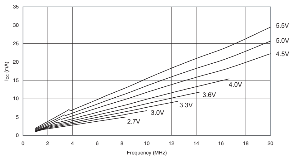
Figure 150. Active Supply Current vs. Frequency (1 MHz - 20 MHz)
