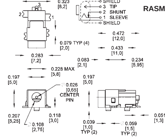
PC BOARD LAYOUT COMPONENT SIDE
