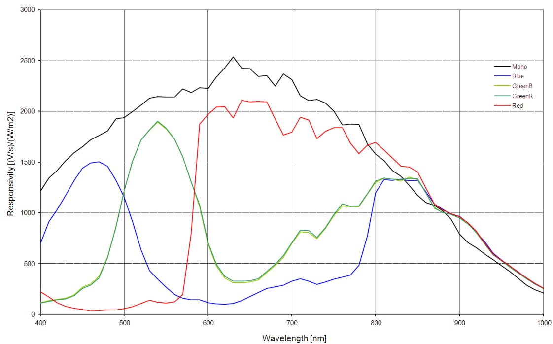
Figure 3. Mono and Color Spectral Response with Micro Lens
